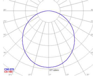
FUTURA K-60x60_45W_D
