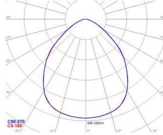
FUTURA K-60x60_45W_mP
