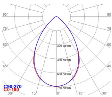
DRAGON 2.0 L-75_190W_4000K
