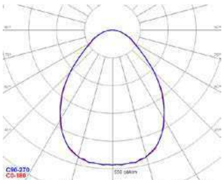
FUTU-NT60x60_-45W_P
