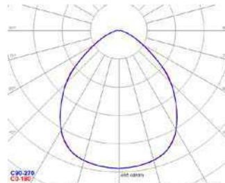
FUTU-NT60x60_-45W_mP
