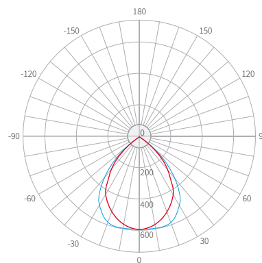
Light distribution curve of the selected fitting SPACE HB 190W cd/klm — C0 - C180 — C90 - C270
